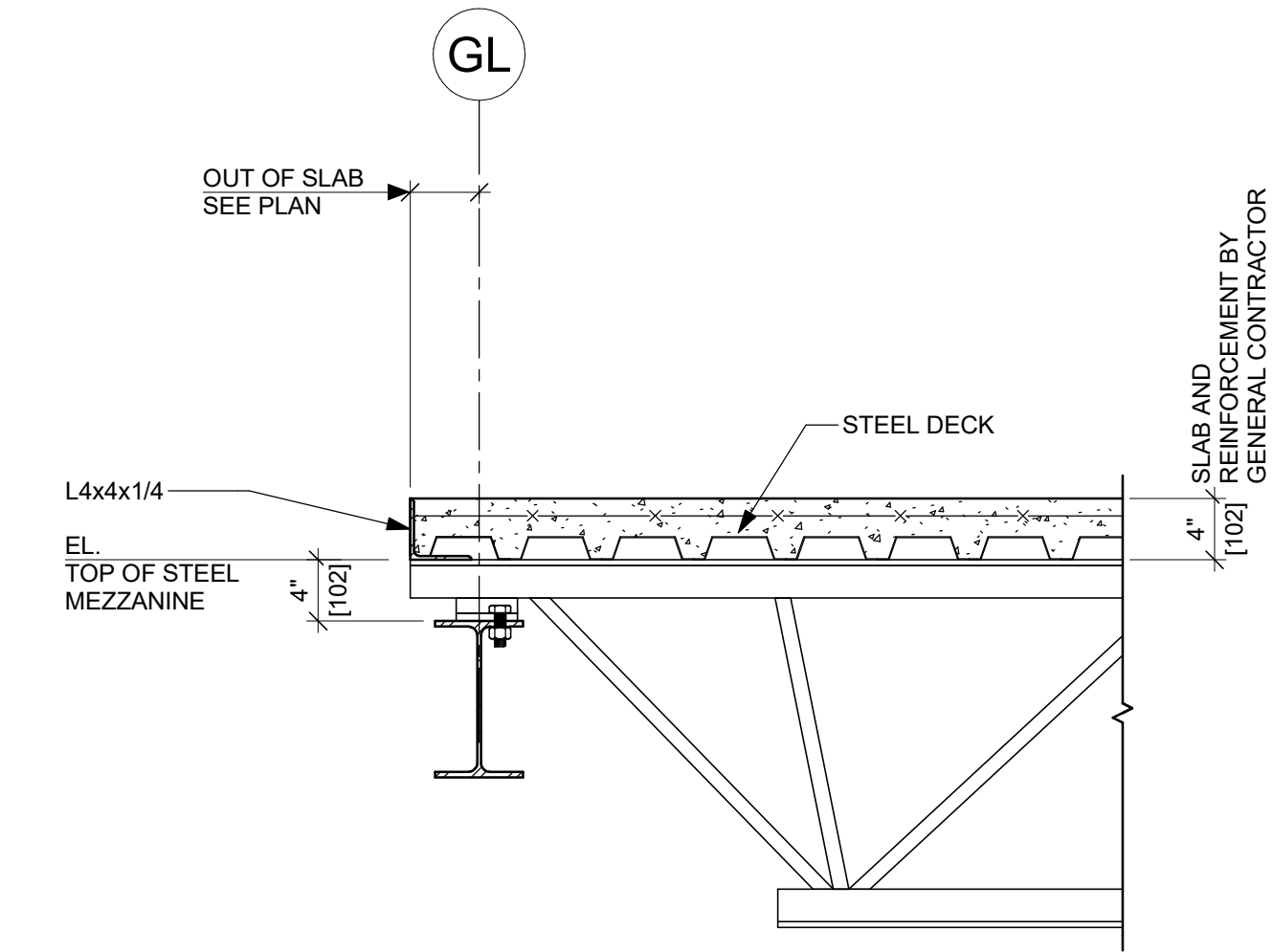
PRELIMINARY SLAB DESIGN 1" = 1'-0"
