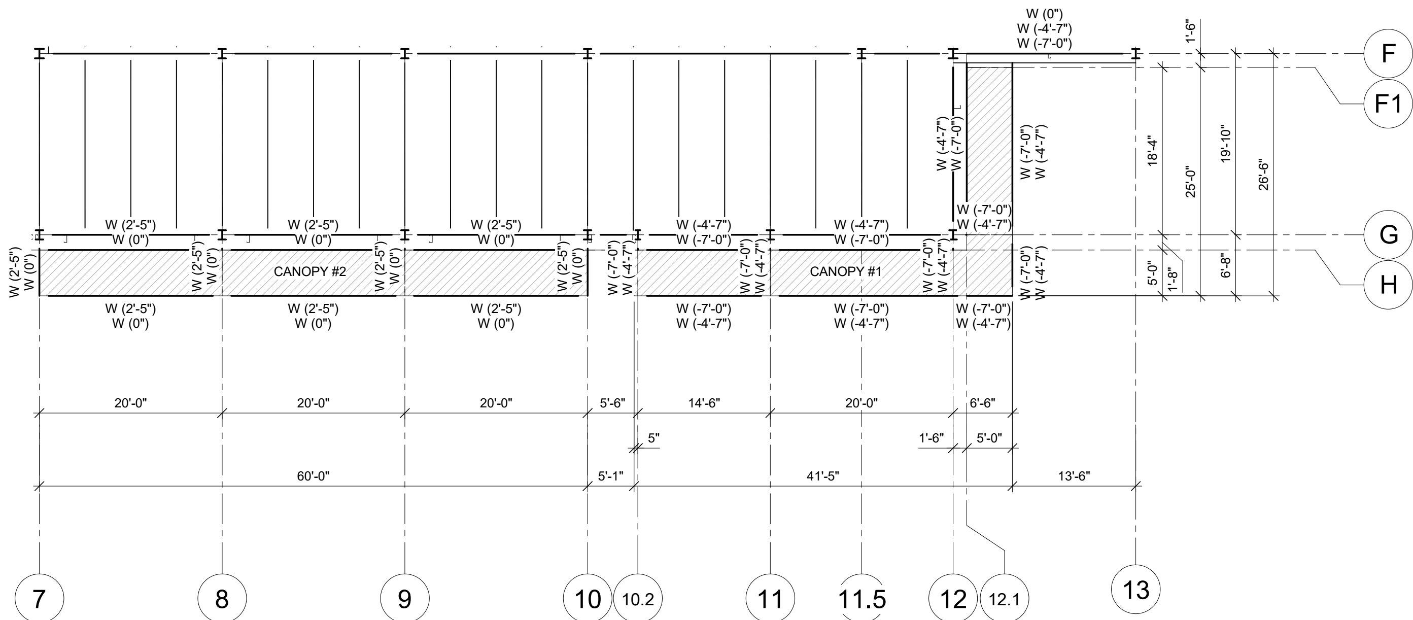
1 CANOPIES PLAN 3/32" = 1'-0"
